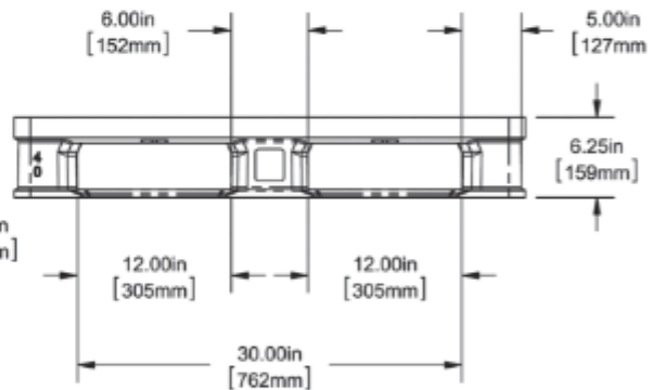
SIDE VIEW - 40"
